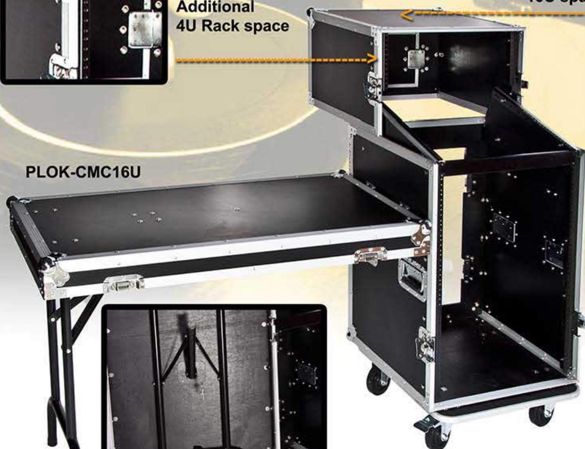
10U space for mixer
